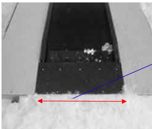
Figure Two. Measurement Guide for Conveyor Belt.
